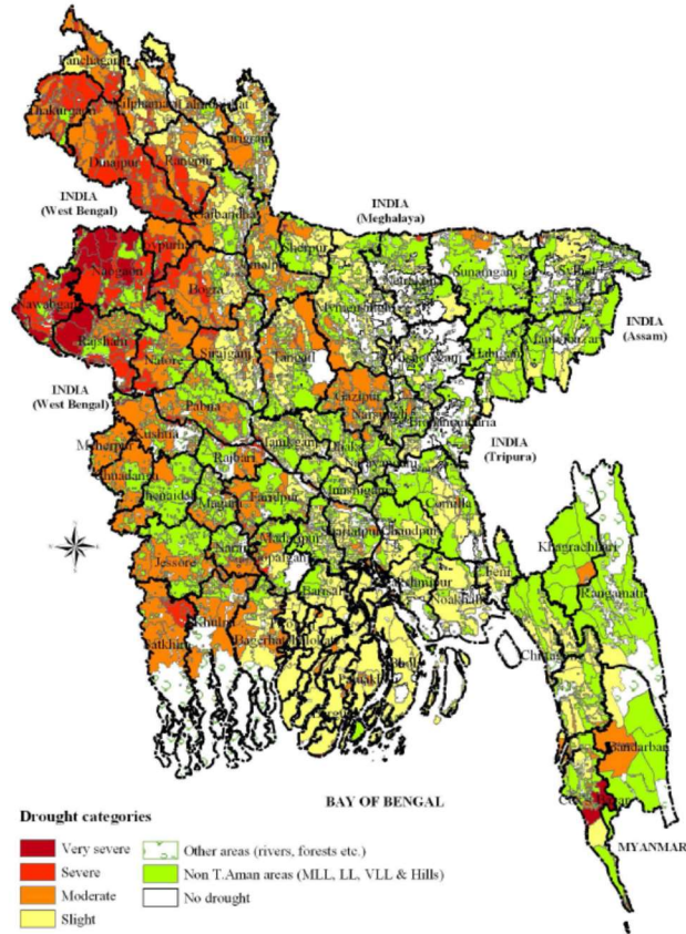
Figure 4: Drought-prone areas in Bangladesh, 2014 Source: M Alimullah Miyan, 2014
