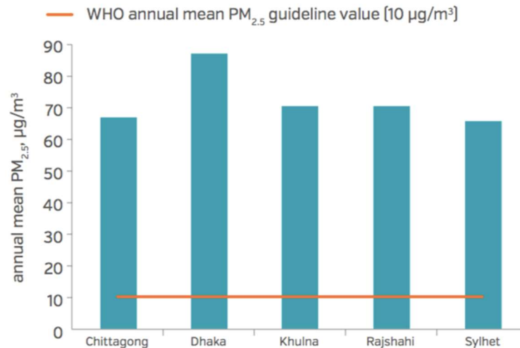
Figure 8: Outdoor air pollution in cities in Bangladesh annual mean pm2.5 (µg/m 3 ) 2013 Source: WHO 2015a
